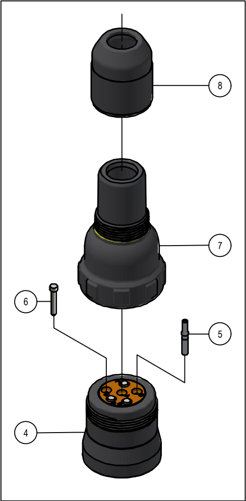
Detail A
