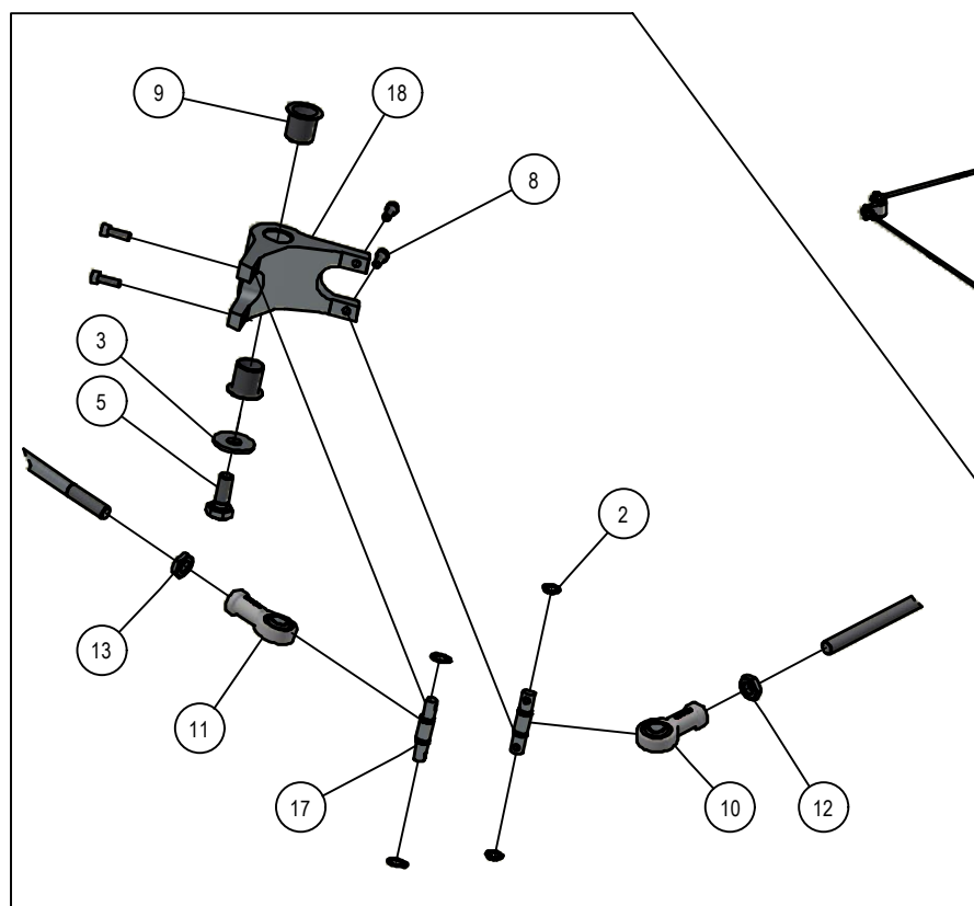
Detail A
