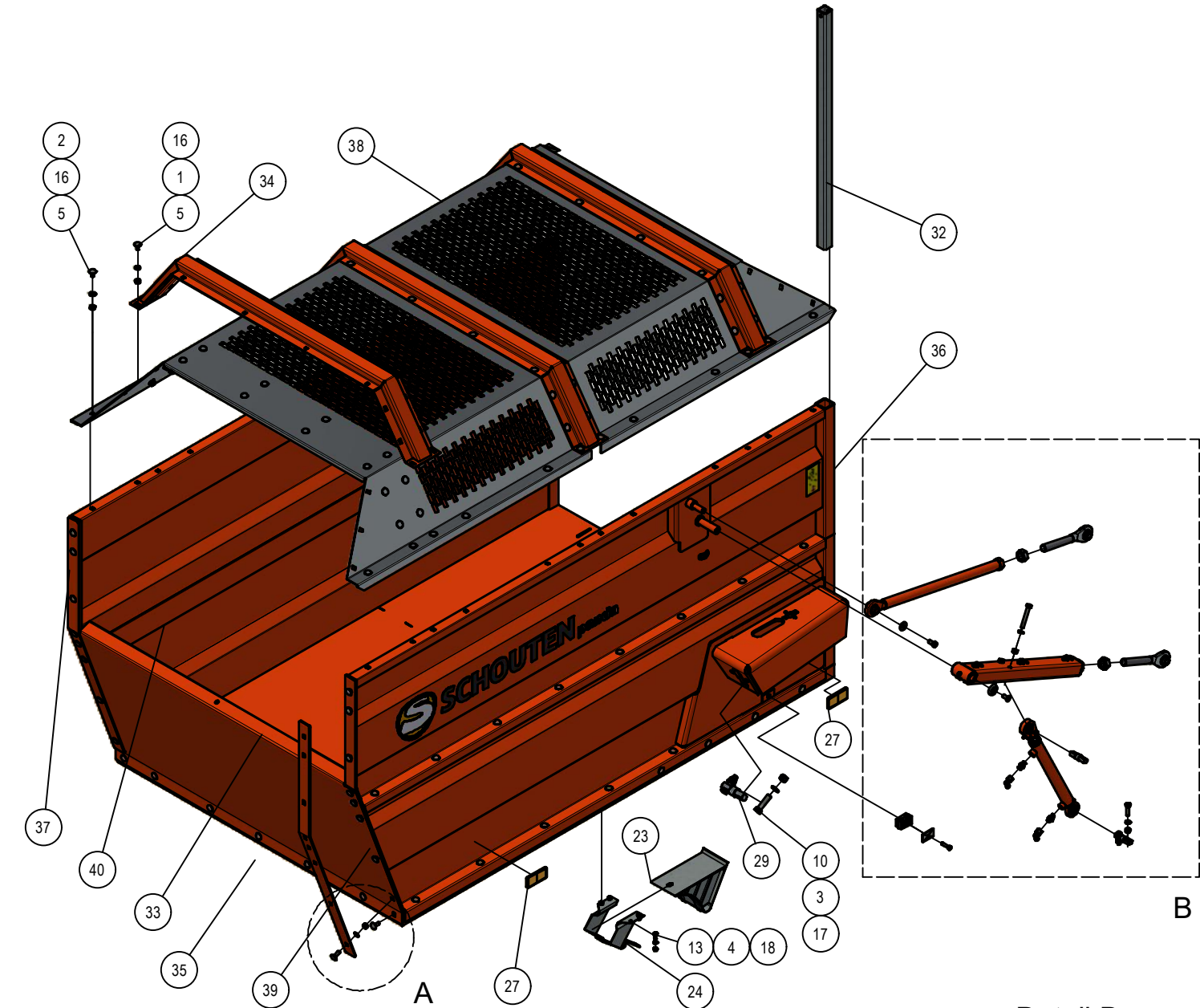
Detail B
