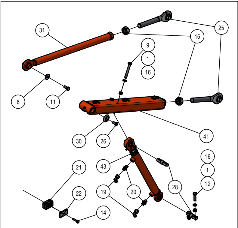
Detail B
