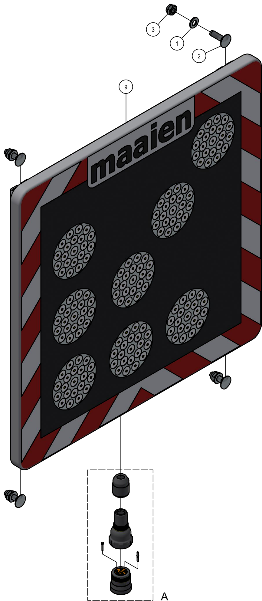
Detail A
